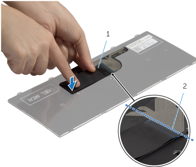
1 keyboard cable
